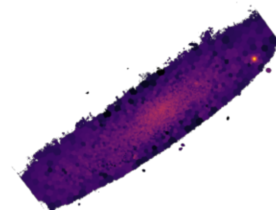
NGC4396
