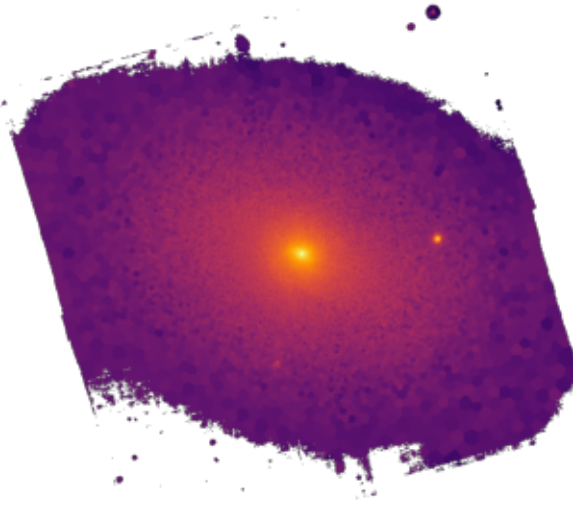
NGC4457
