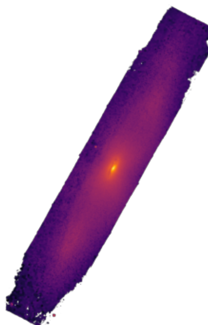
NGC4192
