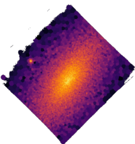
NGC4694
