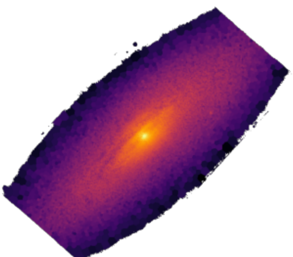
NGC4419
