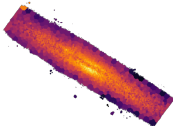
NGC4330
