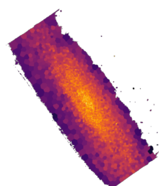
NGC4522
